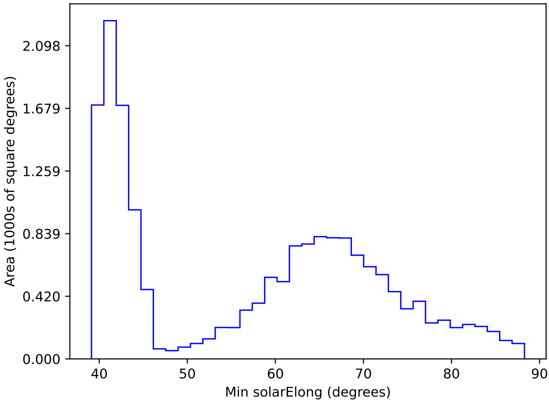
too_elab_r32_d3_gz_v3.4_10yrs WFD r band: Min solarElong
