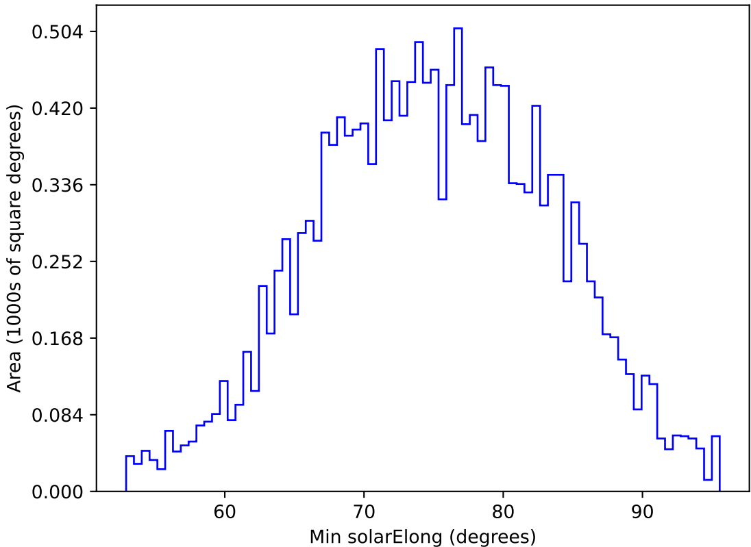
too_elab_r32_d3_gz_v3.4_10yrs WFD g band: Min solarElong
