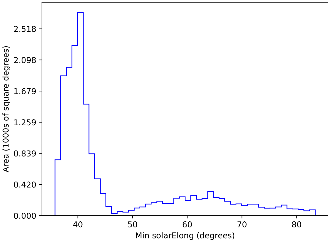
too_elab_r32_d3_gz_v3.4_10yrs WFD all bands: Min solarElong
