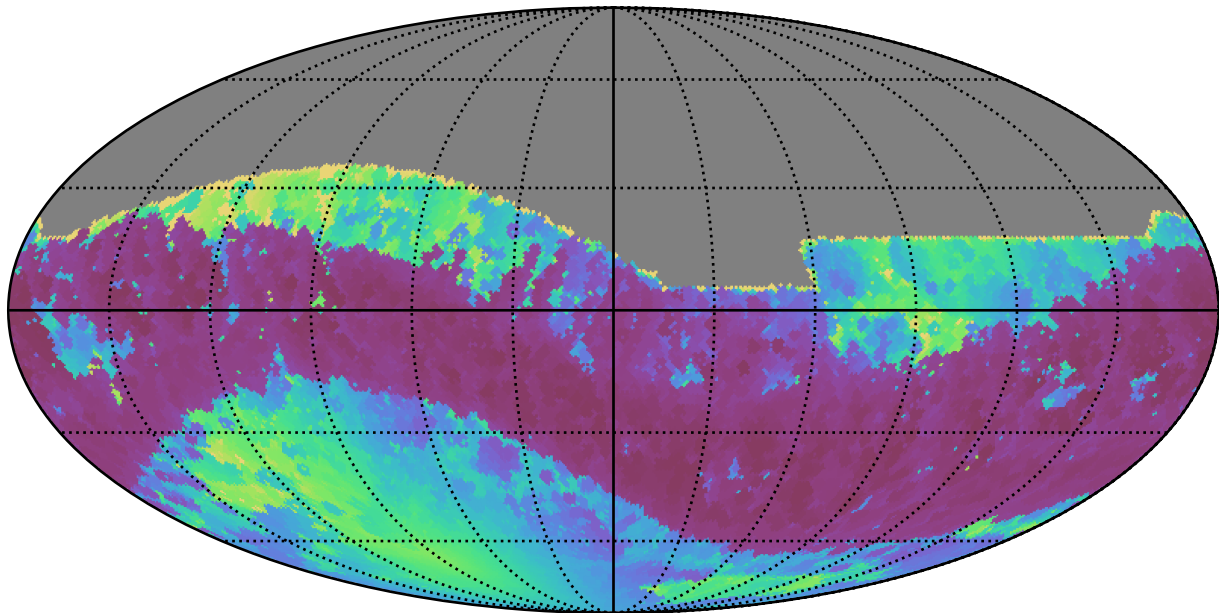
too_elab_r32_d3_gz_v3.4_10yrs All sky z band: Min solarElong
