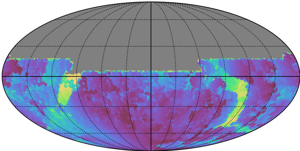
too_elab_r32_d3_gz_v3.4_10yrs All sky u band: Min solarElong
