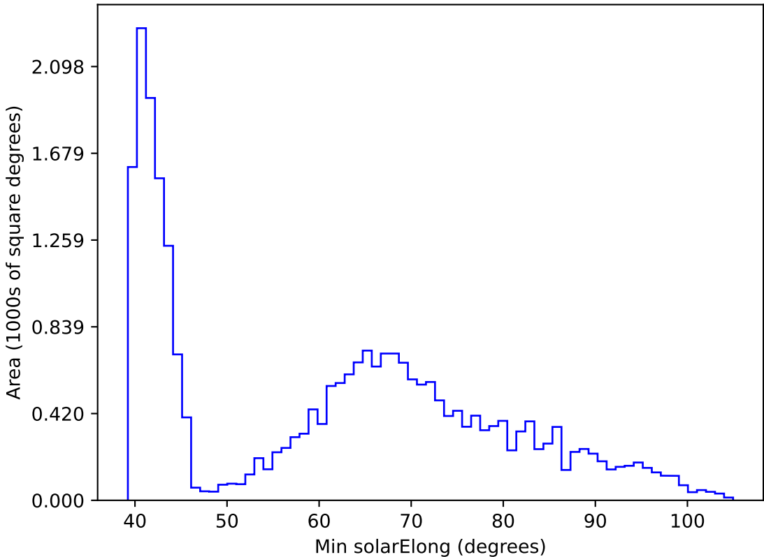
too_elab_r32_d3_gz_v3.4_10yrs All sky r band: Min solarElong
