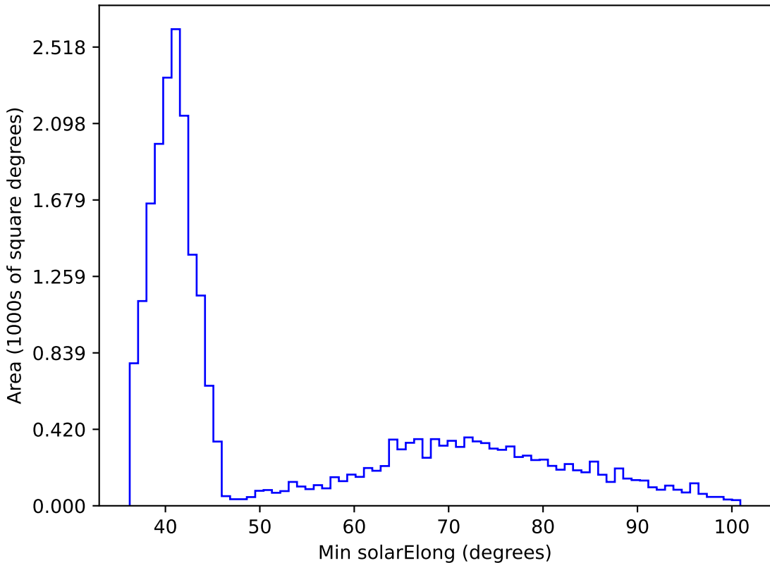
too_elab_r32_d3_gz_v3.4_10yrs All sky i band: Min solarElong
