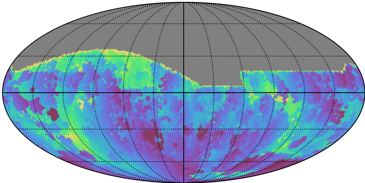
too_elab_r32_d3_gz_v3.4_10yrs All sky g band: Min solarElong
