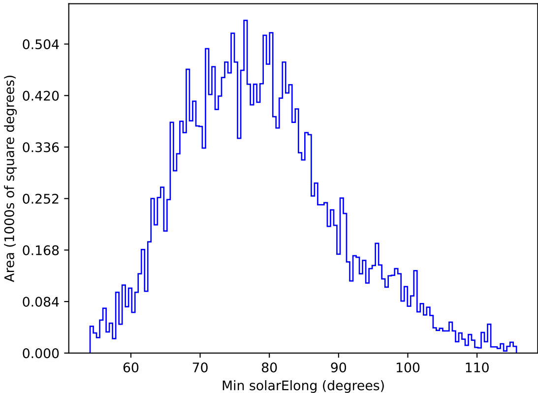
too_elab_r32_d3_gz_v3.4_10yrs All sky g band: Min solarElong
