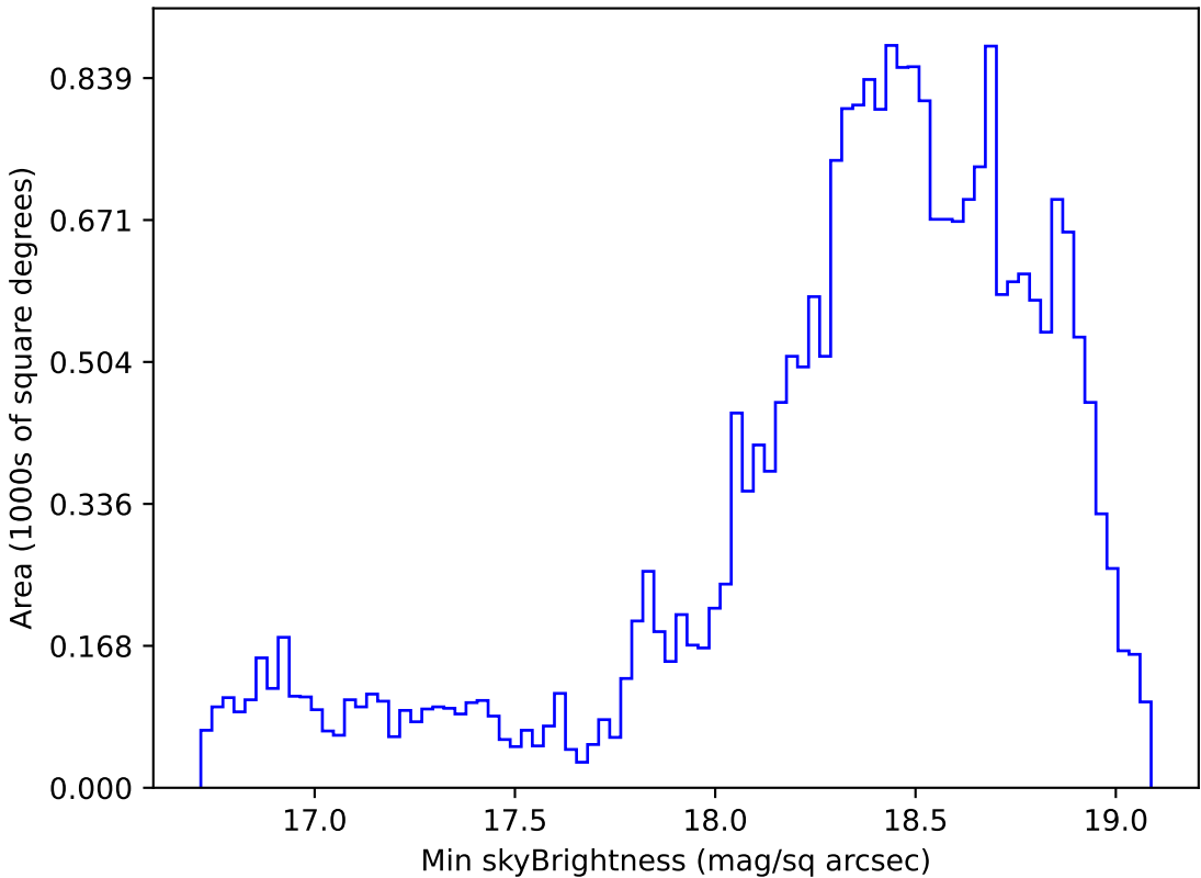
too_elab_r32_d3_gz_v3.4_10yrs Yr 1 z band: Min skyBrightness
