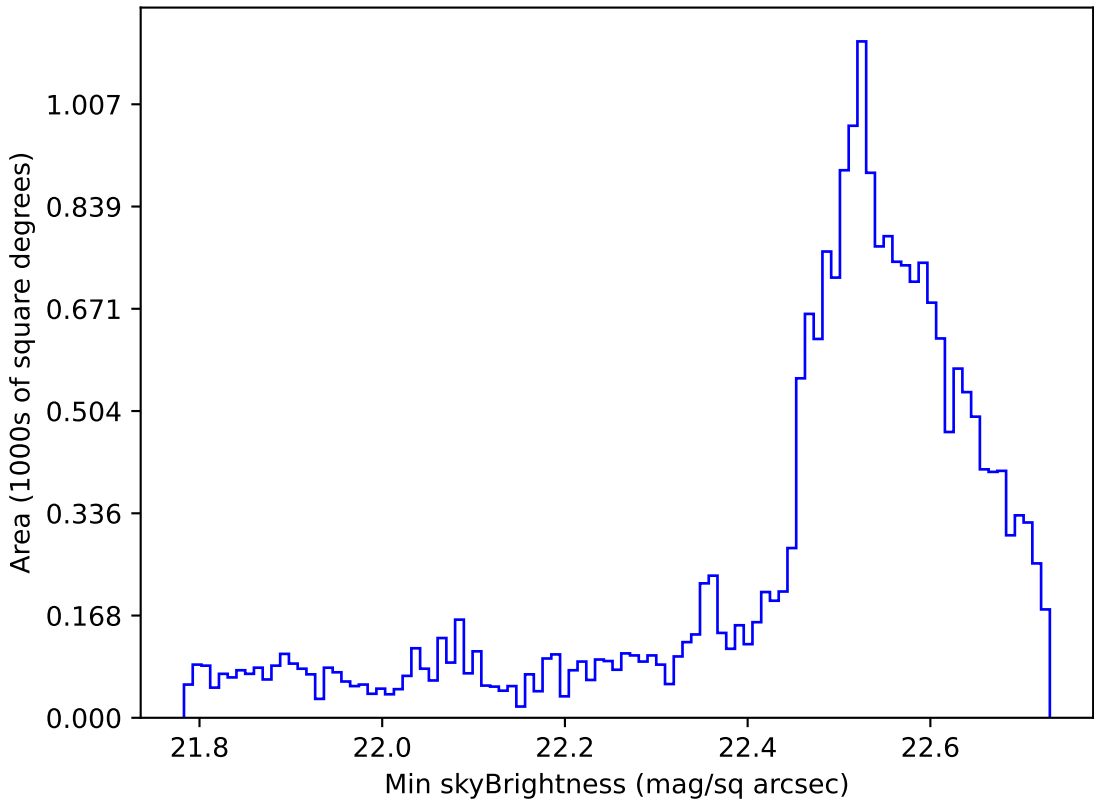
too_elab_r32_d3_gz_v3.4_10yrs Yr 1 u band: Min skyBrightness
