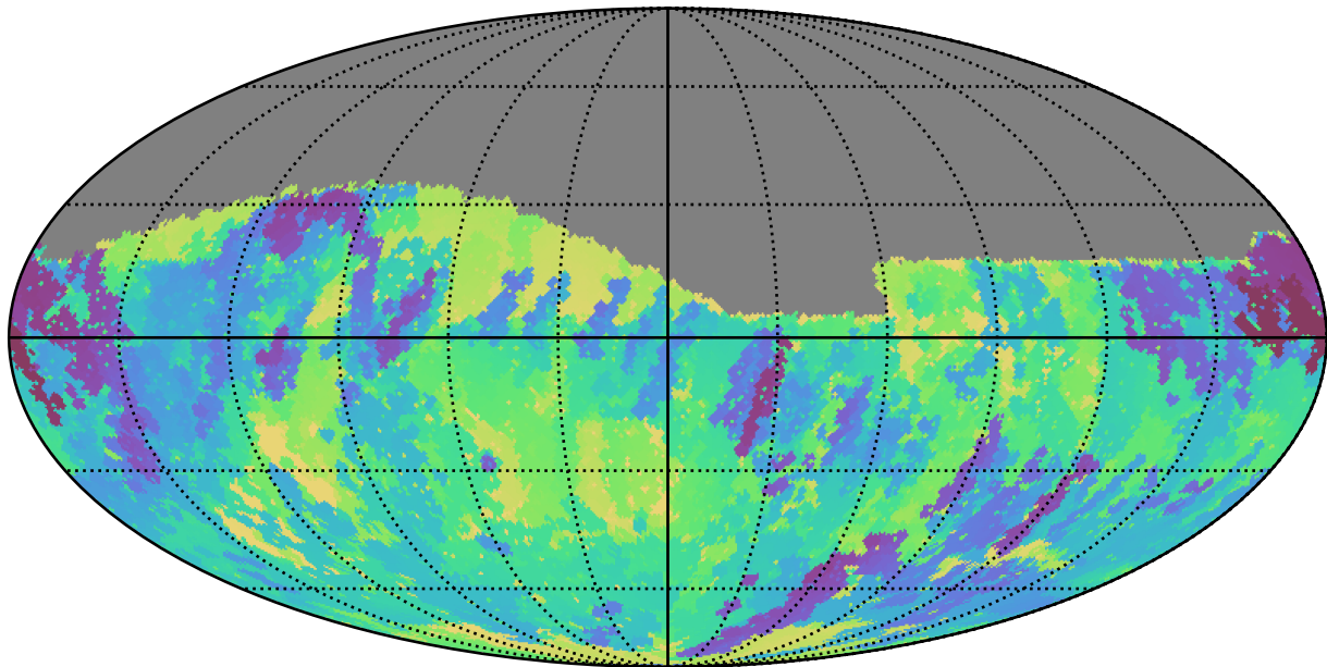
too_elab_r32_d3_gz_v3.4_10yrs Yr 1 r band: Min skyBrightness
