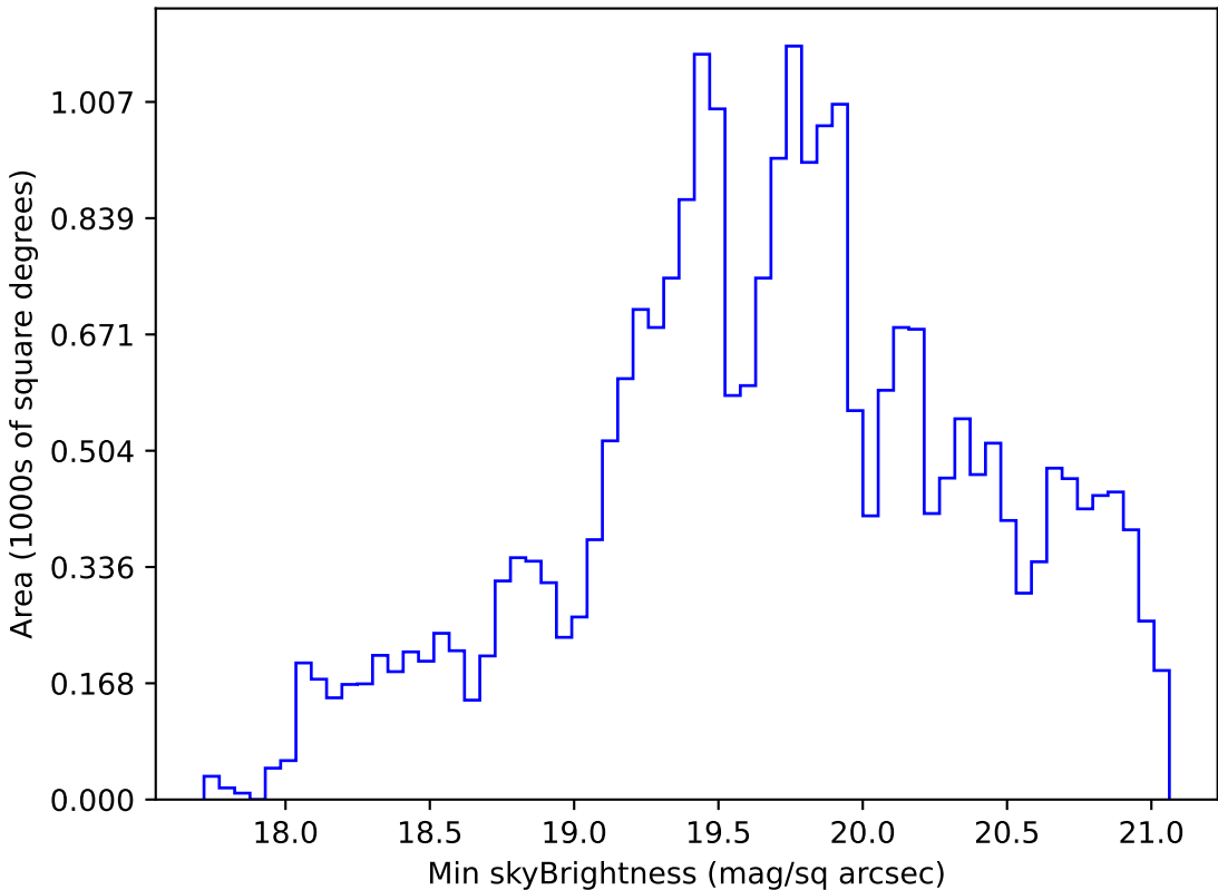
too_elab_r32_d3_gz_v3.4_10yrs Yr 1 r band: Min skyBrightness
