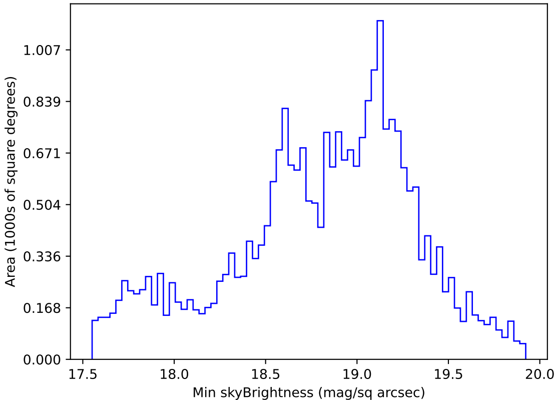
too_elab_r32_d3_gz_v3.4_10yrs Yr 1 i band: Min skyBrightness
