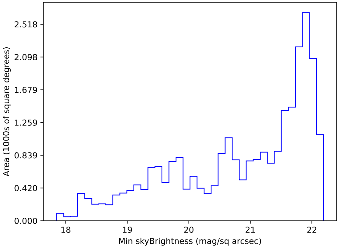
too_elab_r32_d3_gz_v3.4_10yrs Yr 1 g band: Min skyBrightness
