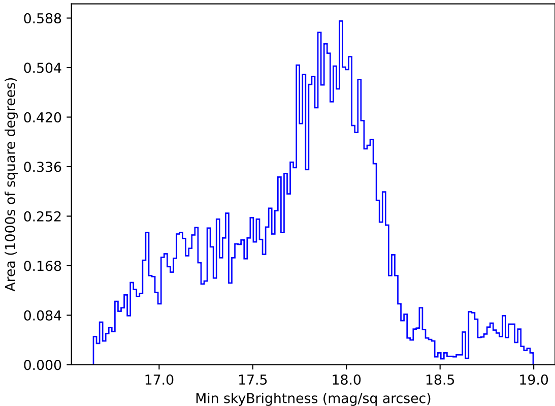
too_elab_r32_d3_gz_v3.4_10yrs Yr 1 all bands: Min skyBrightness
