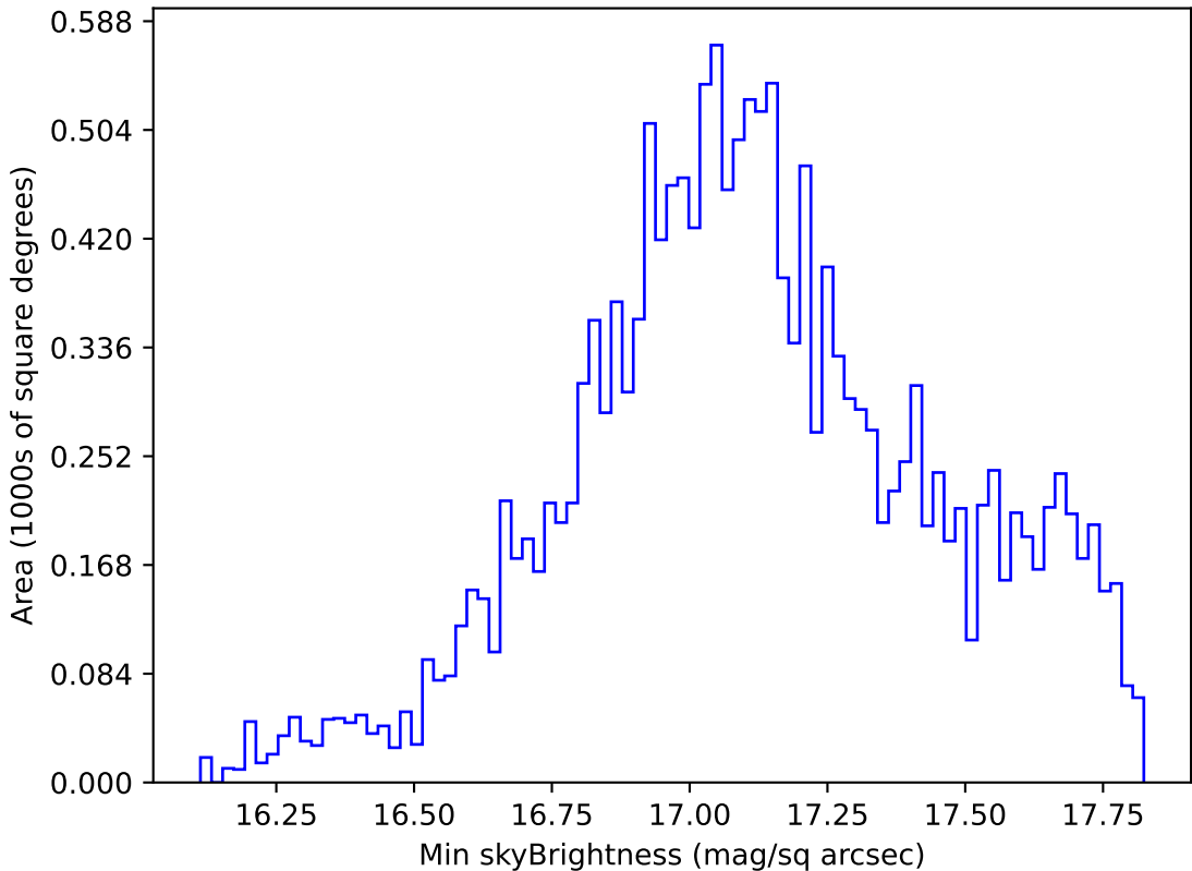
too_elab_r32_d3_gz_v3.4_10yrs WFD y band: Min skyBrightness
