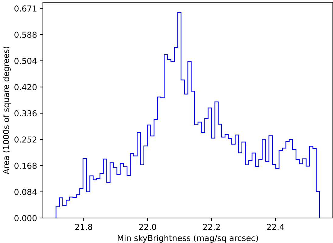
too_elab_r32_d3_gz_v3.4_10yrs WFD u band: Min skyBrightness
