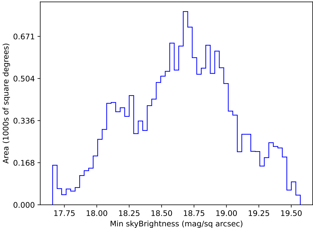
too_elab_r32_d3_gz_v3.4_10yrs WFD r band: Min skyBrightness
