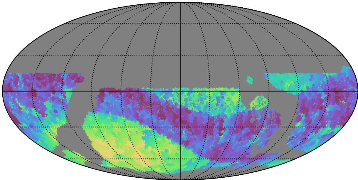
too_elab_r32_d3_gz_v3.4_10yrs WFD i band: Min skyBrightness
