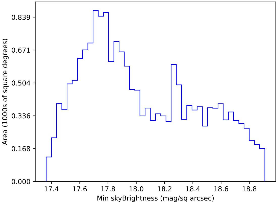
too_elab_r32_d3_gz_v3.4_10yrs WFD i band: Min skyBrightness
