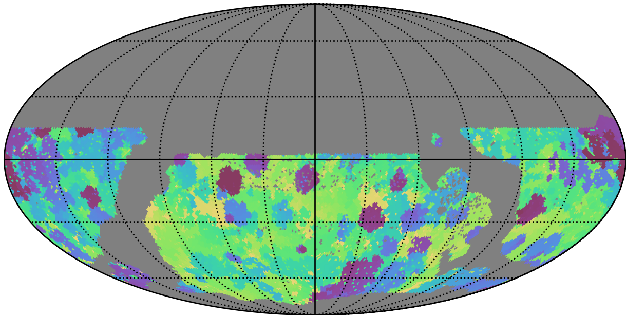
too_elab_r32_d3_gz_v3.4_10yrs WFD g band: Min skyBrightness
