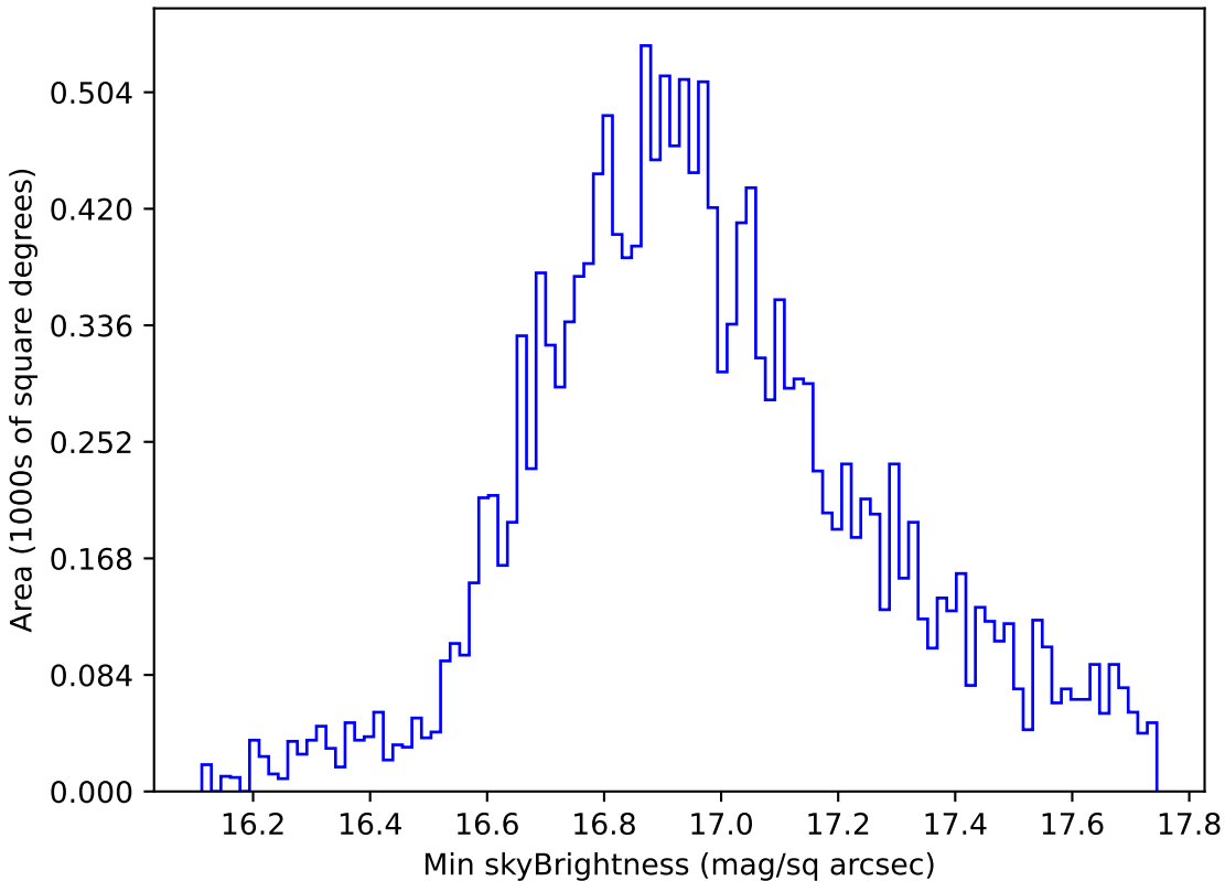
too_elab_r32_d3_gz_v3.4_10yrs WFD all bands: Min skyBrightness
