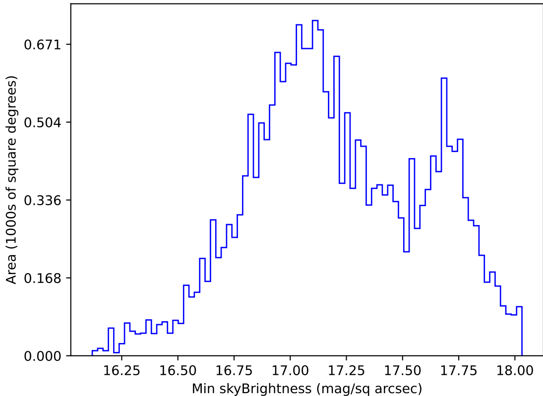
too_elab_r32_d3_gz_v3.4_10yrs All sky y band: Min skyBrightness
