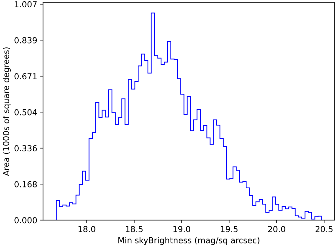
too_elab_r32_d3_gz_v3.4_10yrs All sky r band: Min skyBrightness
