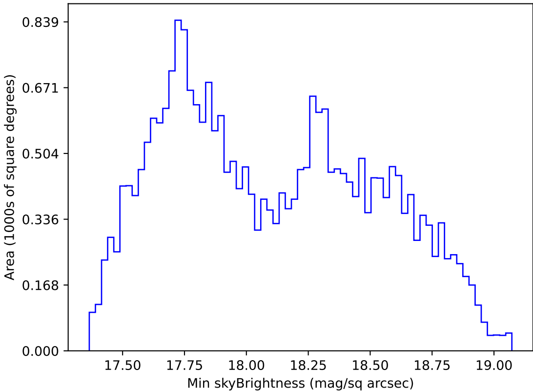
too_elab_r32_d3_gz_v3.4_10yrs All sky i band: Min skyBrightness
