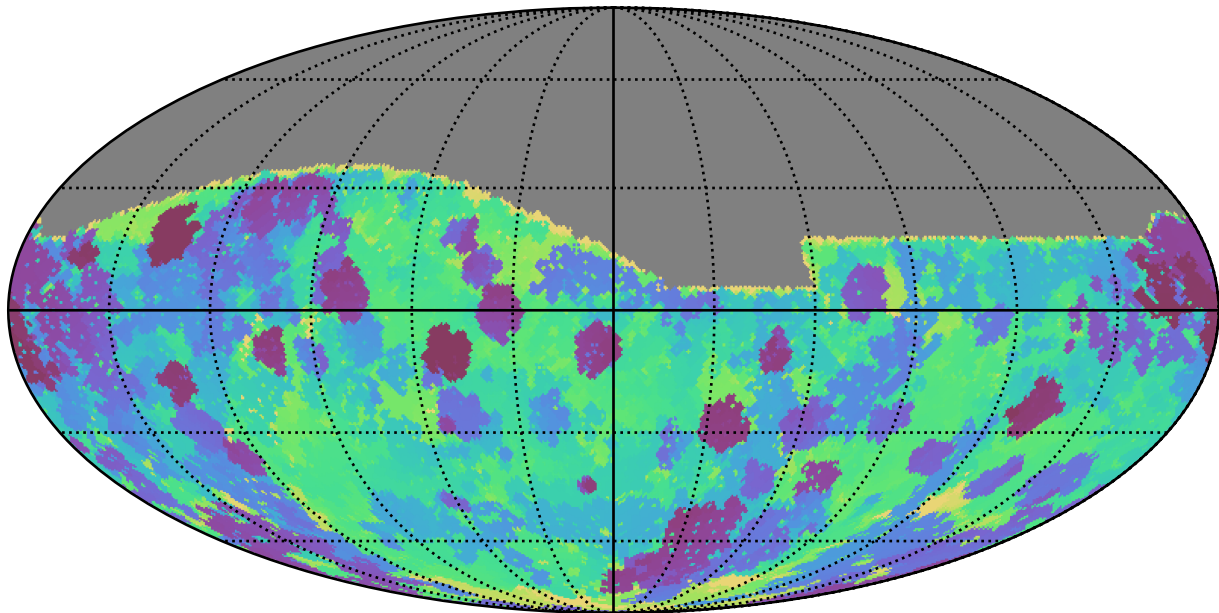
too_elab_r32_d3_gz_v3.4_10yrs All sky g band: Min skyBrightness
