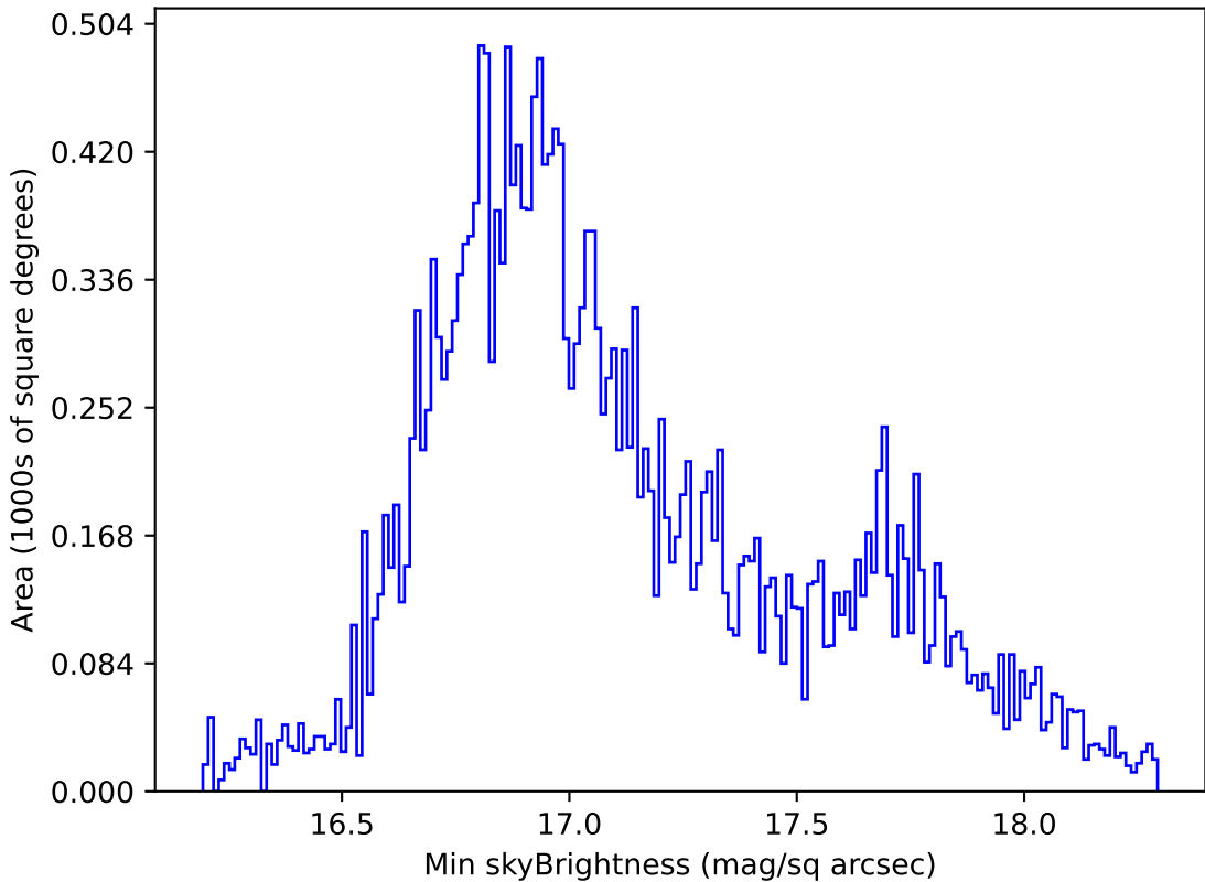
too_elab_r32_d3_gz_v3.4_10yrs All sky all bands: Min skyBrightness
