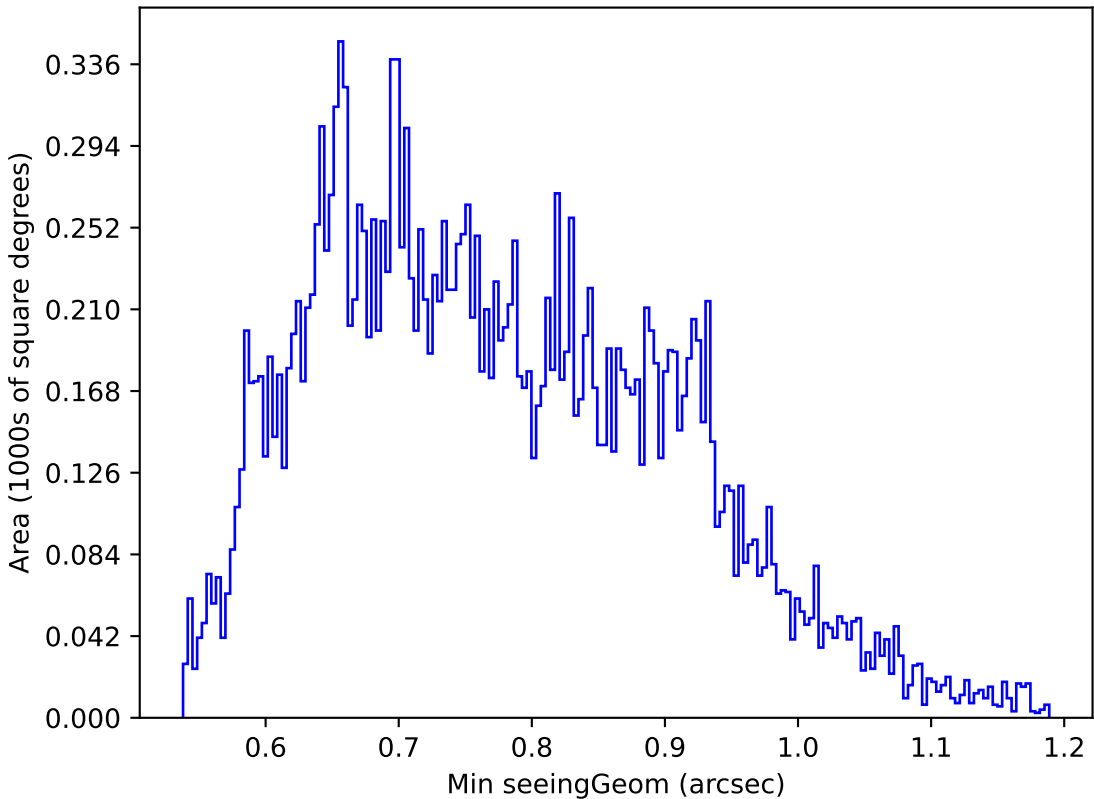
too_elab_r32_d3_gz_v3.4_10yrs Yr 1 u band: Min seeingGeom
