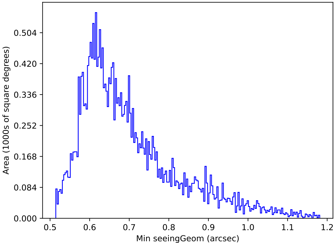
too_elab_r32_d3_gz_v3.4_10yrs Yr 1 g band: Min seeingGeom
