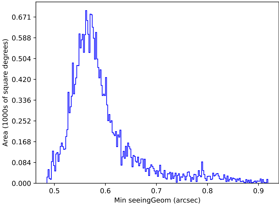
too_elab_r32_d3_gz_v3.4_10yrs Yr 1 all bands: Min seeingGeom
