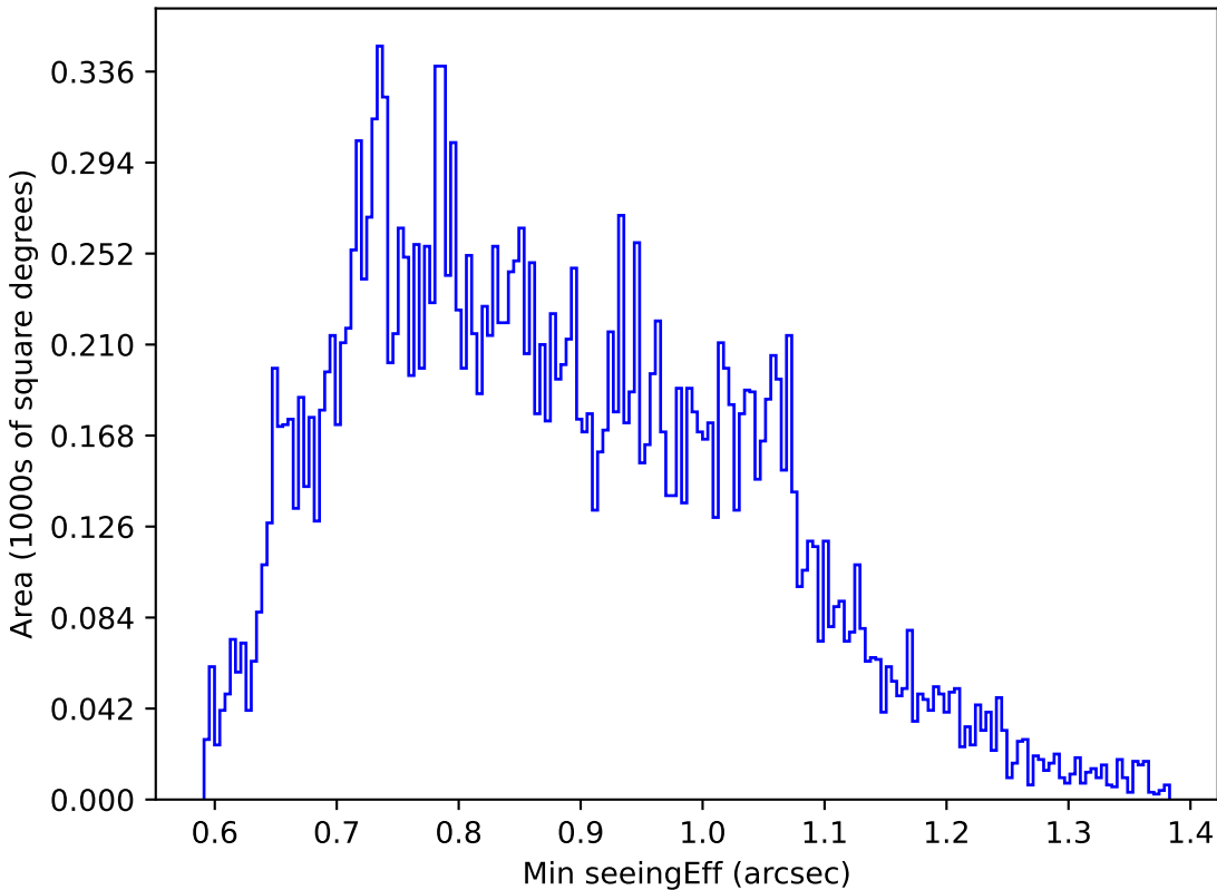
too_elab_r32_d3_gz_v3.4_10yrs Yr 1 u band: Min seeingEff
