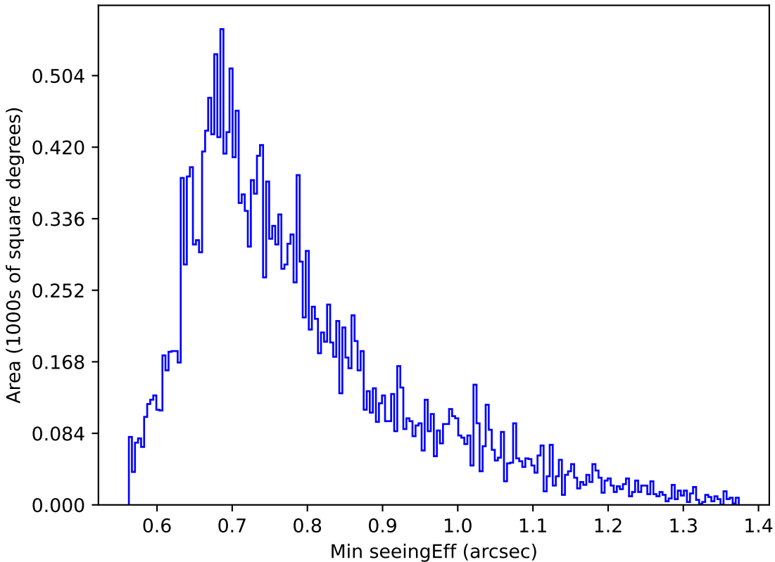
too_elab_r32_d3_gz_v3.4_10yrs Yr 1 g band: Min seeingEff
