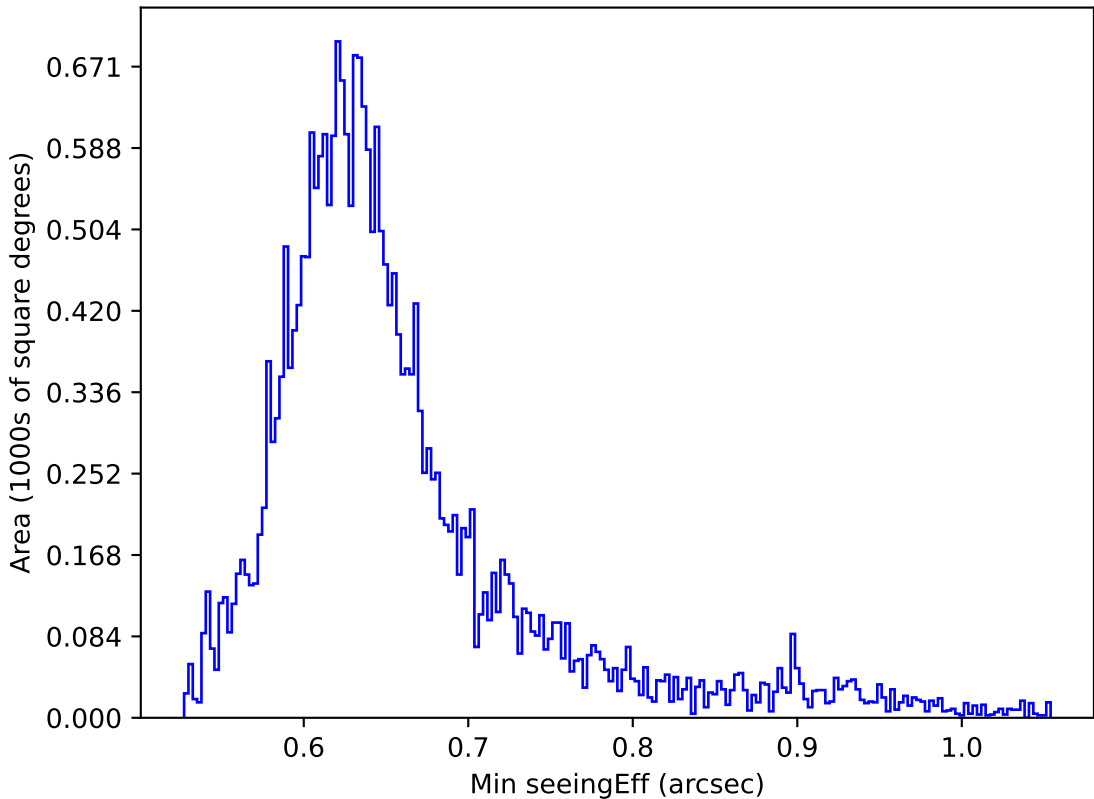
too_elab_r32_d3_gz_v3.4_10yrs Yr 1 all bands: Min seeingEff
