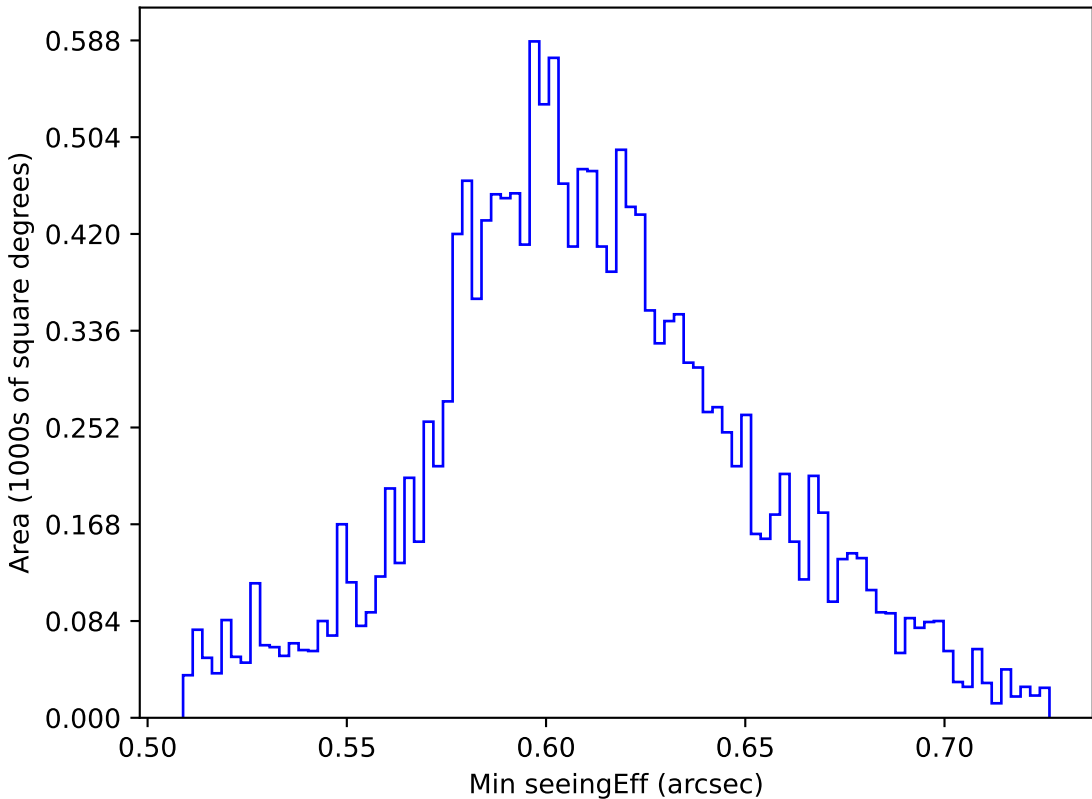
too_elab_r32_d3_gz_v3.4_10yrs WFD z band: Min seeingEff
