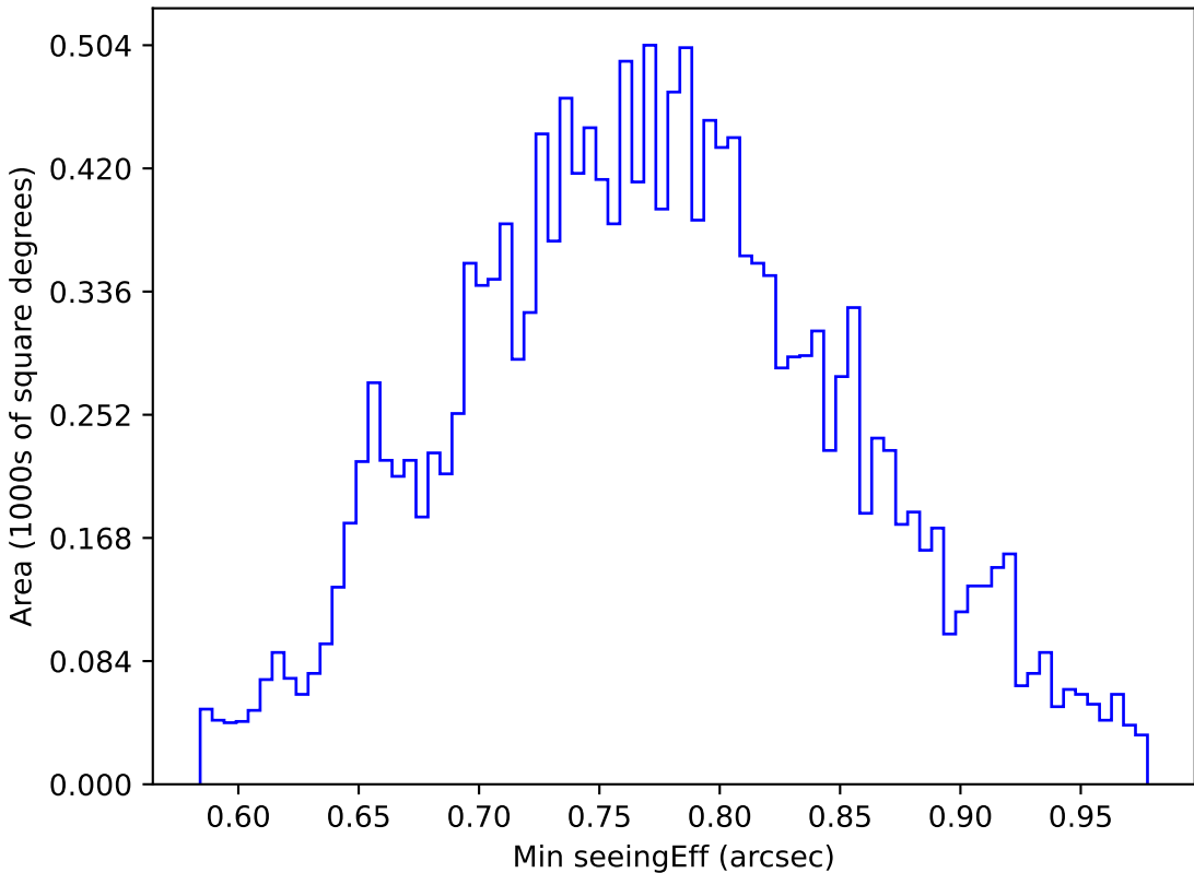
too_elab_r32_d3_gz_v3.4_10yrs WFD u band: Min seeingEff
