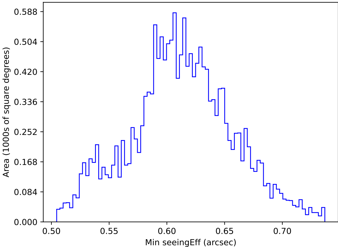
too_elab_r32_d3_gz_v3.4_10yrs WFD r band: Min seeingEff
