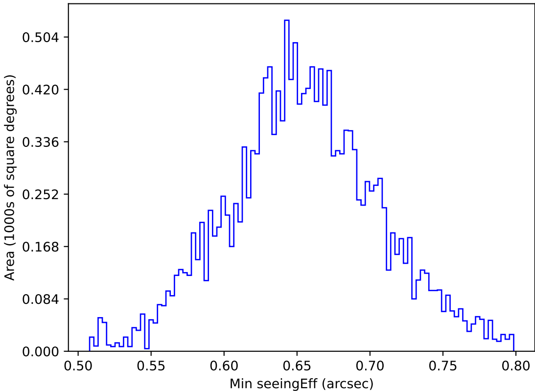
too_elab_r32_d3_gz_v3.4_10yrs WFD g band: Min seeingEff
