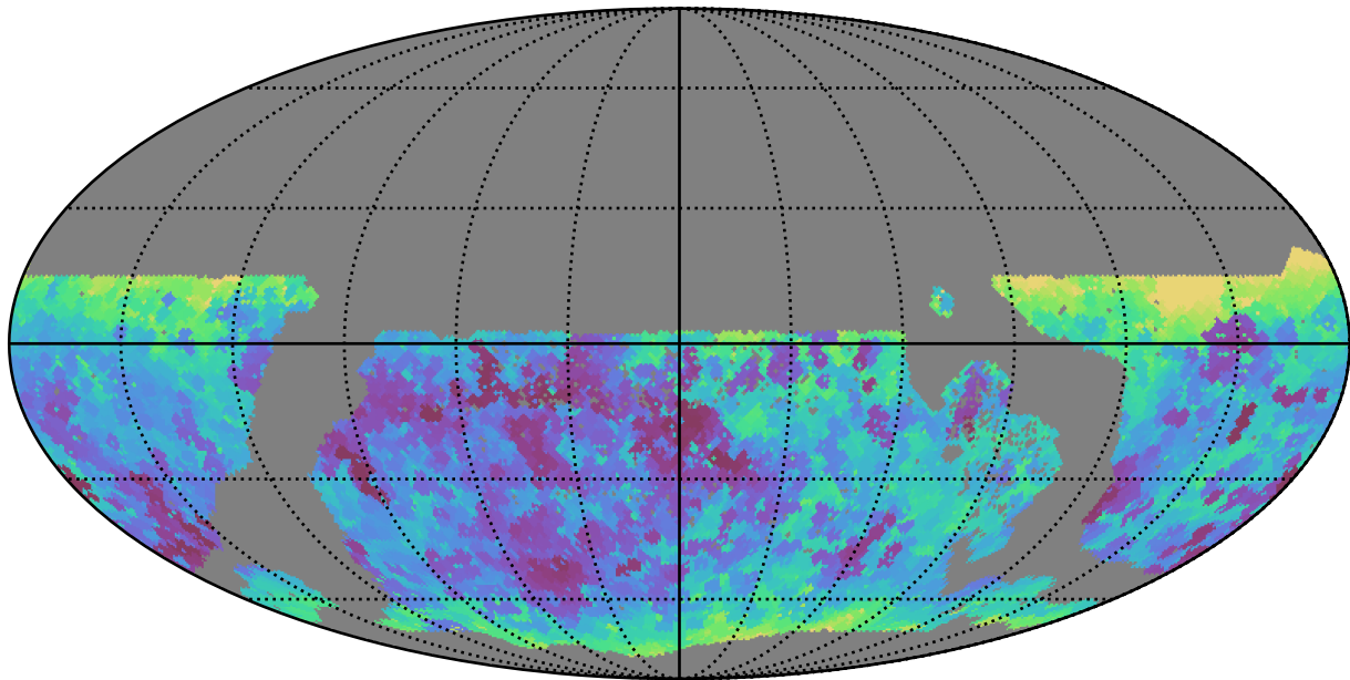
too_elab_r32_d3_gz_v3.4_10yrs WFD all bands: Min seeingEff
