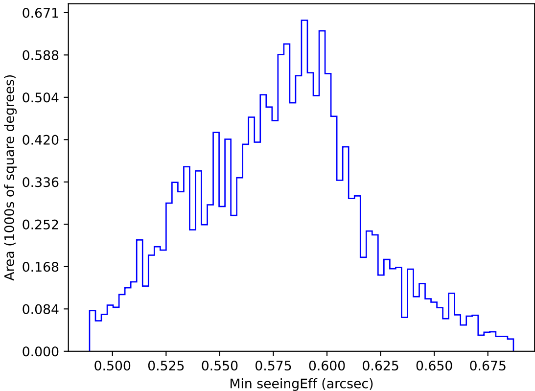
too_elab_r32_d3_gz_v3.4_10yrs WFD all bands: Min seeingEff
