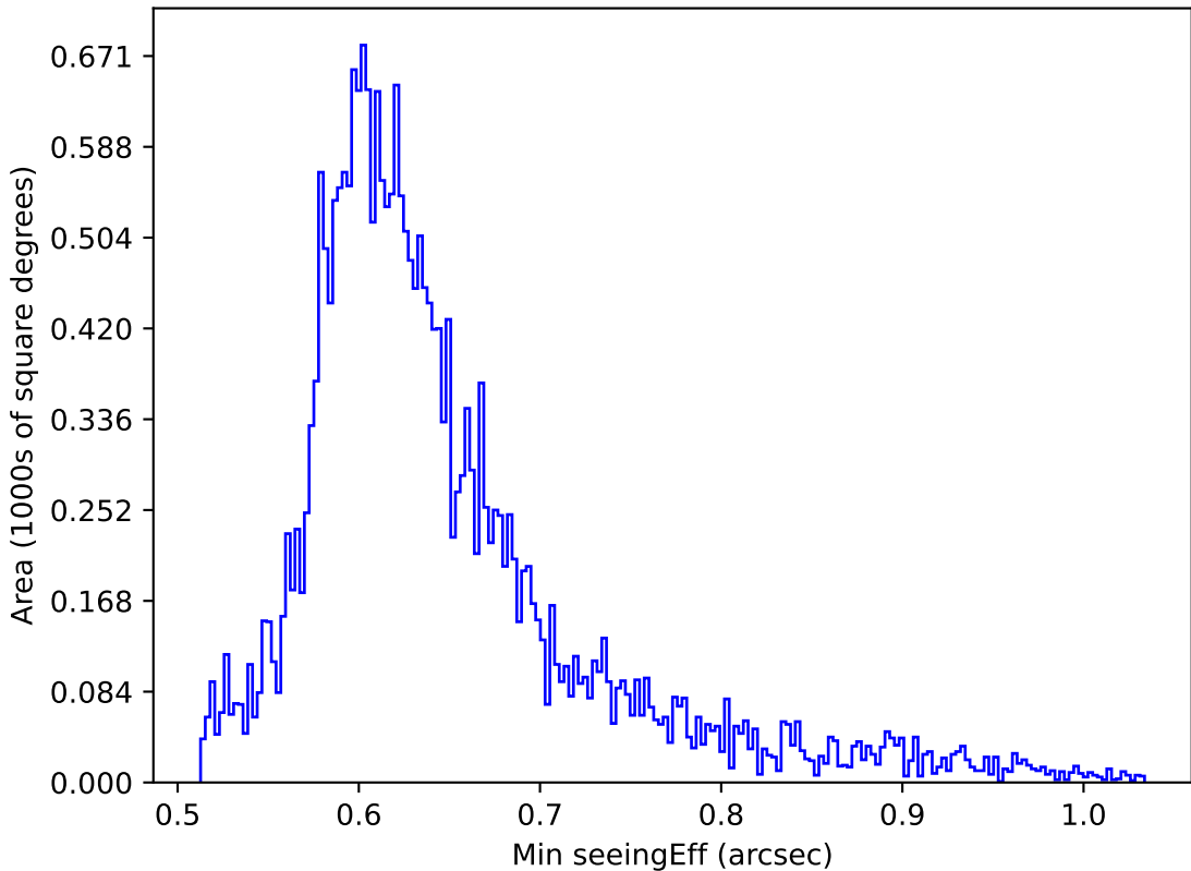
too_elab_r32_d3_gz_v3.4_10yrs All sky z band: Min seeingEff
