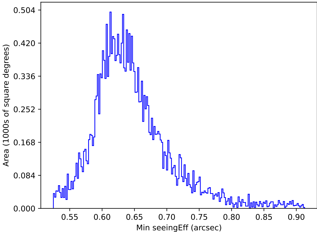
too_elab_r32_d3_gz_v3.4_10yrs All sky y band: Min seeingEff
