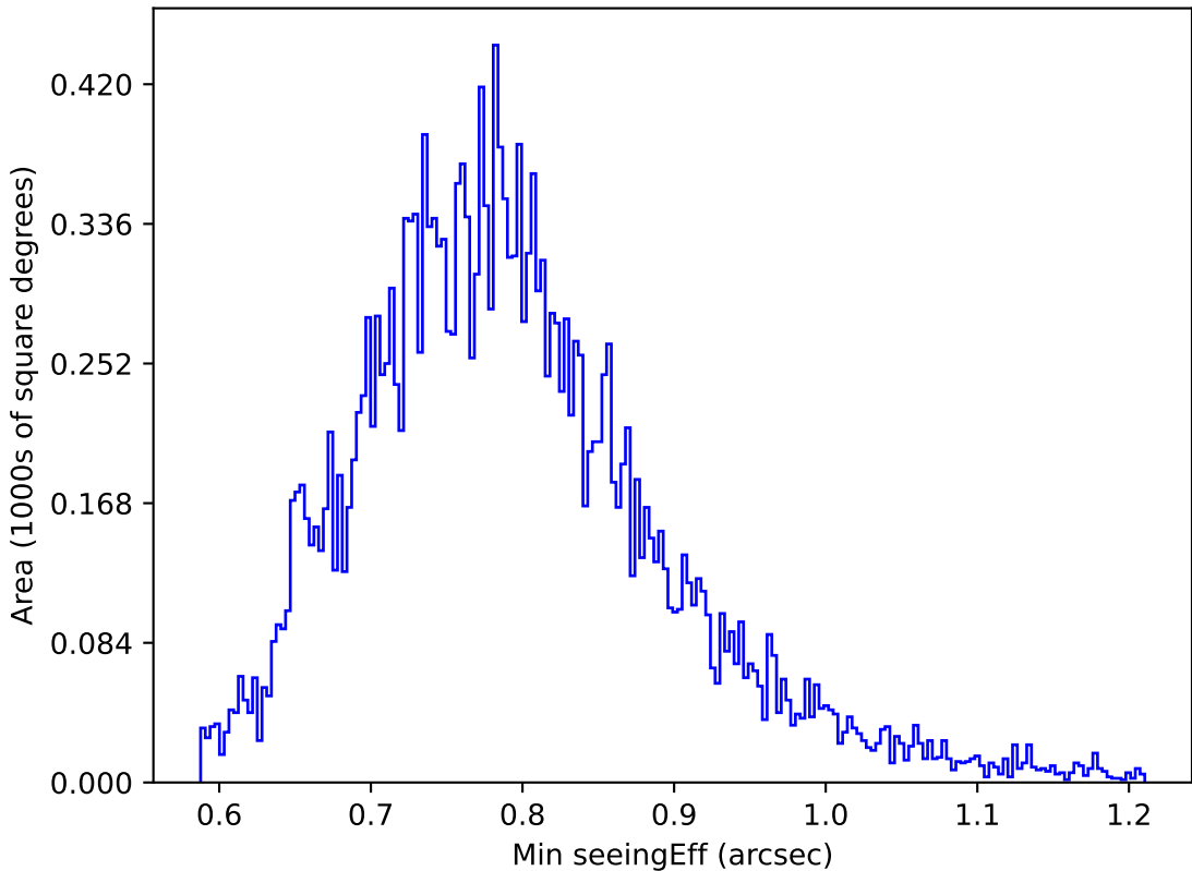
too_elab_r32_d3_gz_v3.4_10yrs All sky u band: Min seeingEff
