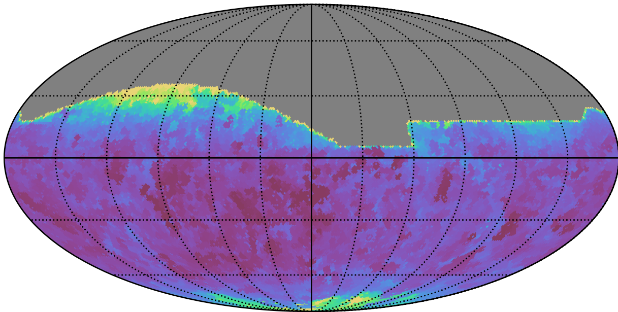
too_elab_r32_d3_gz_v3.4_10yrs All sky r band: Min seeingEff
