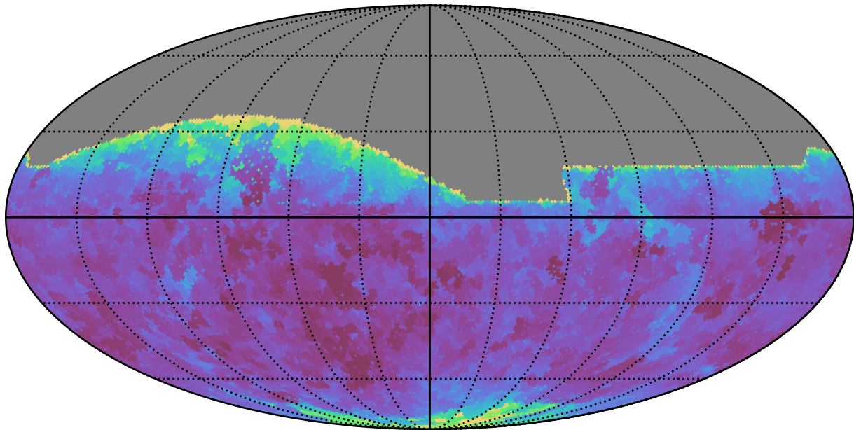
too_elab_r32_d3_gz_v3.4_10yrs All sky i band: Min seeingEff
