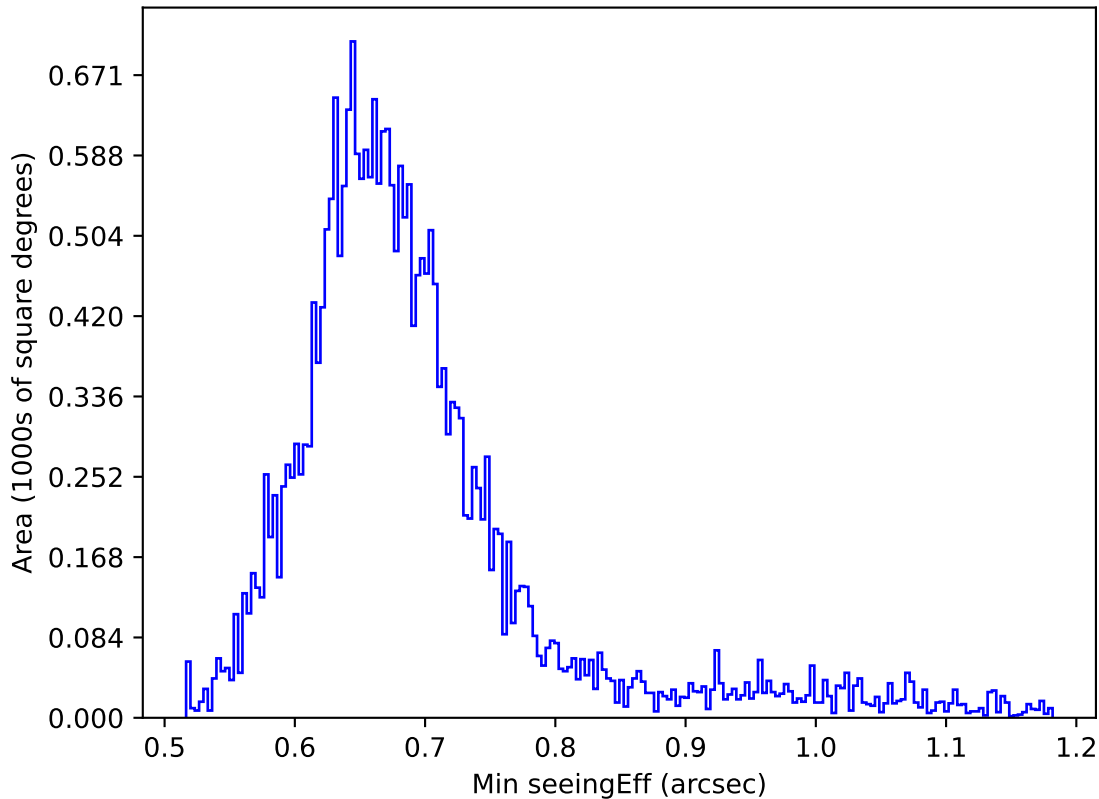
too_elab_r32_d3_gz_v3.4_10yrs All sky g band: Min seeingEff
