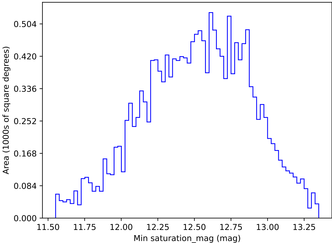
too_elab_r32_d3_gz_v3.4_10yrs WFD r band: Min saturation_mag
