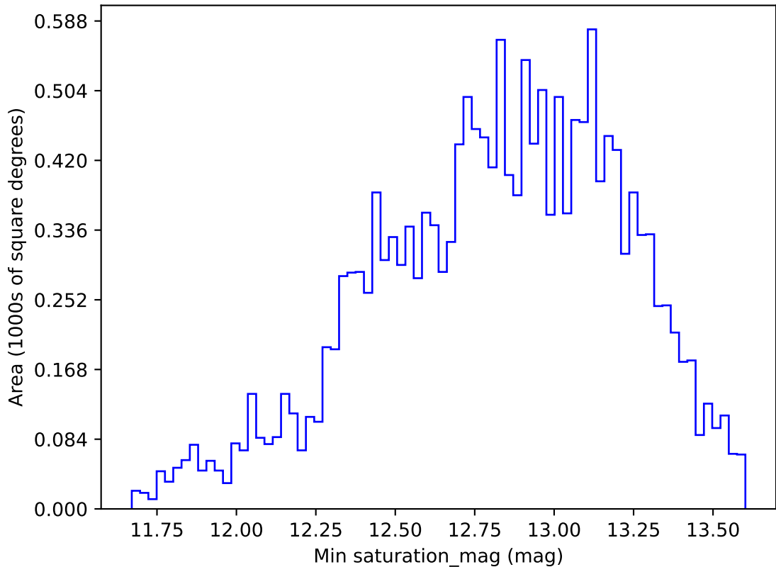
too_elab_r32_d3_gz_v3.4_10yrs WFD g band: Min saturation_mag
