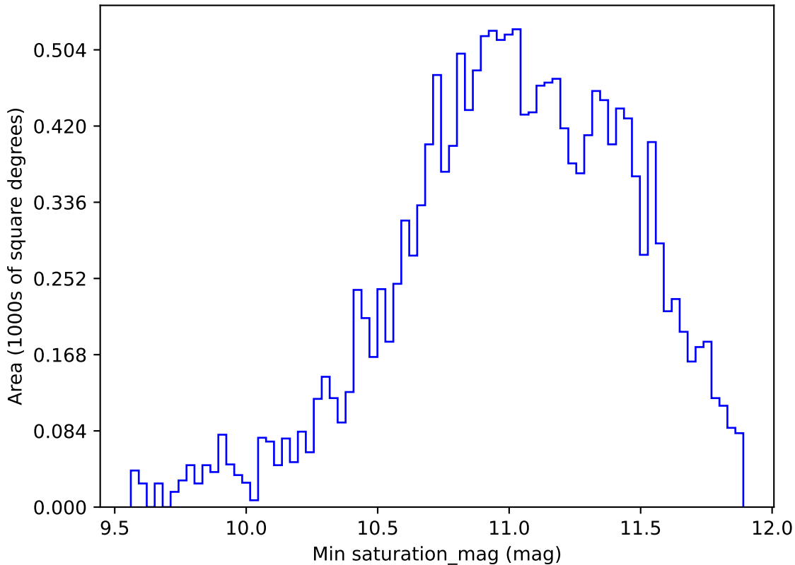
too_elab_r32_d3_gz_v3.4_10yrs WFD all bands: Min saturation_mag
