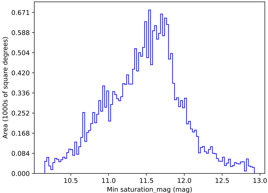
too_elab_r32_d3_gz_v3.4_10yrs All sky u band: Min saturation_mag
